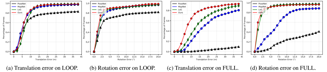
Figure 6: Cumulative distributions of the mean position and orientation errors of PoseNet, MapNet, LsG, and our method on the Oxford RobotCar LOOP and FULL scenes. X-axis and y-axis denote the error and the percentage of frames, respectively.
