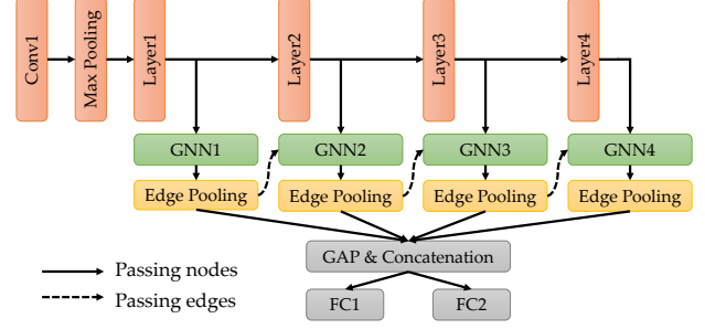
Figure 4: Multi-level modeling. ResNet34 [15] is integrated with GNNs for iterative feature processing at four levels. After each GNN block, an edge pooling is performed to discard redundant connections. Fused features from four GNN blocks are passed through the GAP (global average pooling) layer, concatenated along the channel dimension, and fed into two FC (fully connected) layers for position and orientation prediction, respectively.
