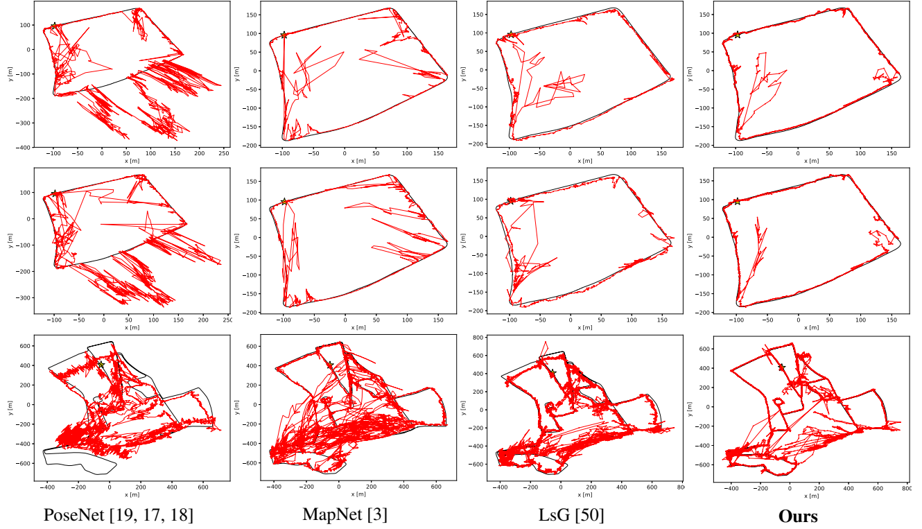
Figure 5: Trajectories of PoseNet, MapNet, LsG, and our model on the LOOP1 (top), LOOP2 (middle), and FULL1 scenes (bottom) of the Oxford RobotCar dataset [24]. The red and black lines indicate predicted and ground truth poses, respectively.
