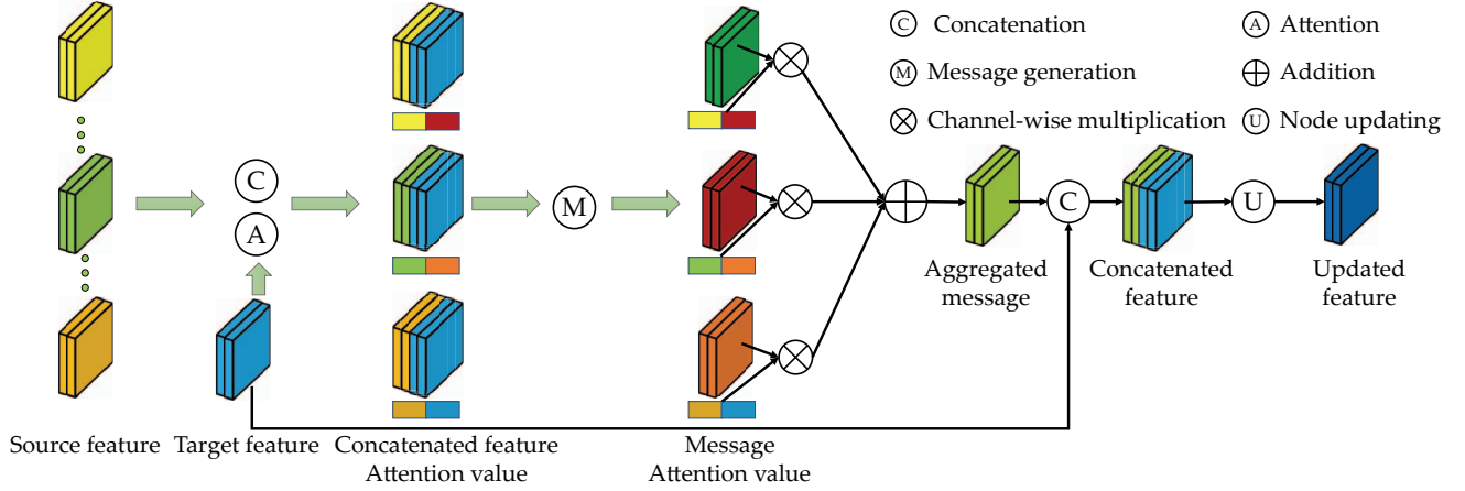
Figure 3: The pipeline of message passing and node updating. Each source feature concatenated with the target one is utilized to generate the message which is then re-weighted along the channel dimension for selection. Messages from all source features are aggregated by adding pixel-wise values and concatenated with the target feature for the final node updating.
