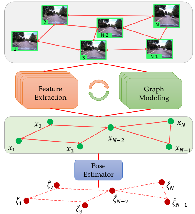
Figure 1: Overview of our framework. We construct a graph with nodes representing observations of different view-points. CNNs and GNNs are exploited for feature extraction and message exchange, respectively. The two processes are executed iteratively at multiple levels with edges dynamically adjusted to retain the most important connections. Enhanced feature of each node is fed into the pose estimator for absolute pose prediction. The preserved edges are utilized to build additional constraints in the training process.
