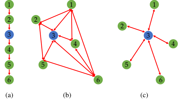
Figure 2: Graph structure. Previous methods [3, 9, 50] focus mainly on the temporal consistency by adding connections between consecutive frames (a). In contrast, we initialize the graph with dense connections (b), so that even temporally distant views can contribute to each other (c).
